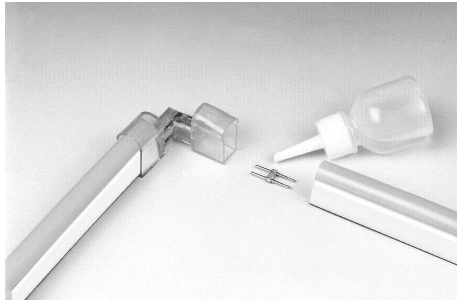
L-connector
